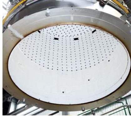
▲ Tangential layout with 12 burners in three different levels. Each burner has a capacity of 150 kW; one burner for H 2 and lubricant residue post combustion. All are equipped with individual heat exchangers.
