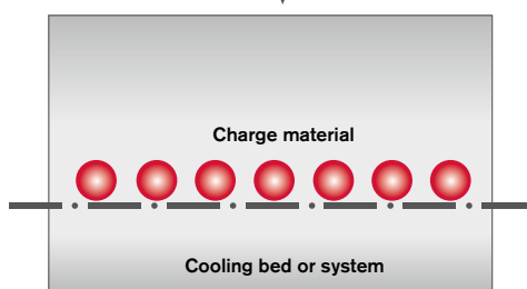
Radiant cooling with or without quenching in air, \text{H}_2\text{O} , air + \text{H}_2\text{O} or \text{H}_2\text{O} -polymer emulsion
